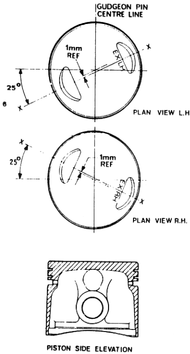
FIG. 1. PISTON CROWN MODIFICATION
