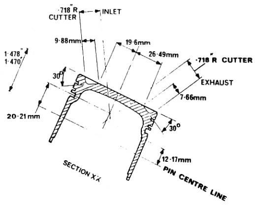
FIG. 1. PISTON CROWN MODIFICATION
