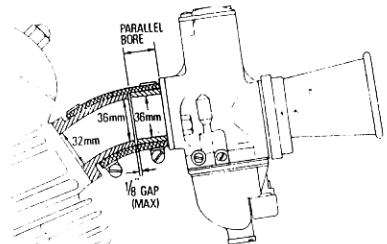
FIG. 4. CARBURETTOR MOUNTING
